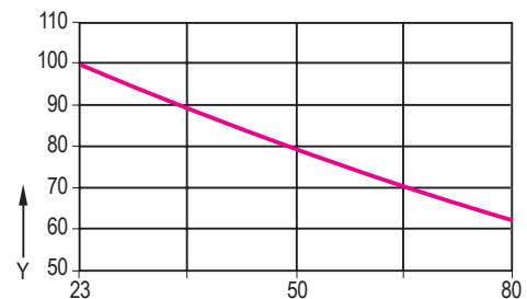
Y = 抗拉强度百分比 Percentage tensile strength [%] X = 温度 Temperature [°C]
